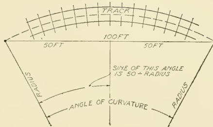
Fig. 129. Graphical Determination of Track Curvature
